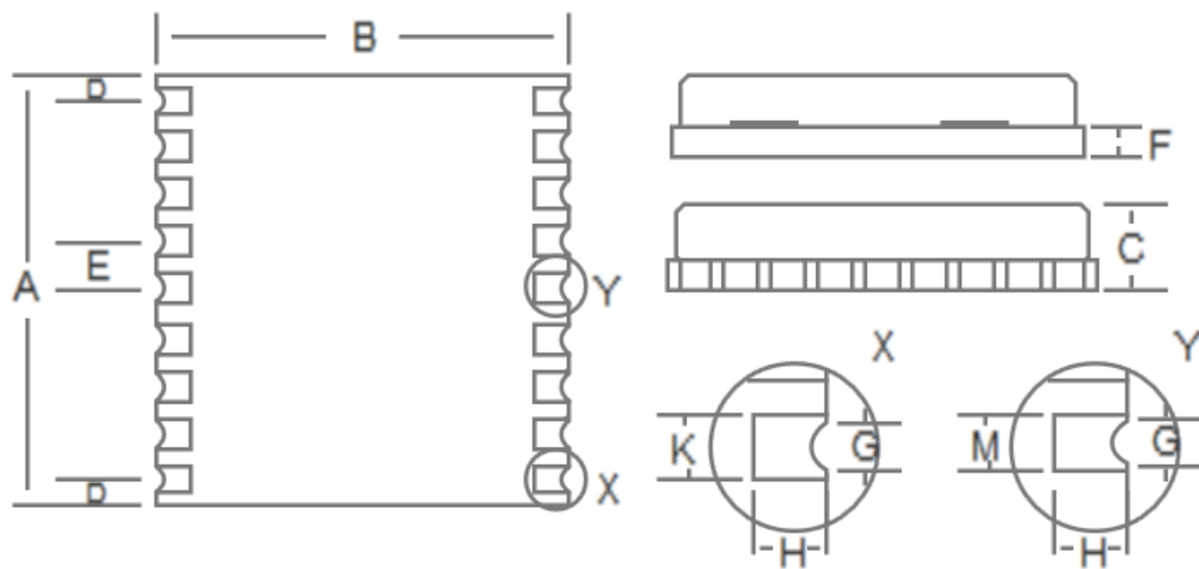
Figure 3-1 Mechanical Layout
