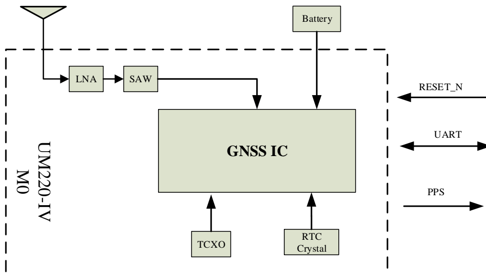
Figure 1-2 Structure Chart
